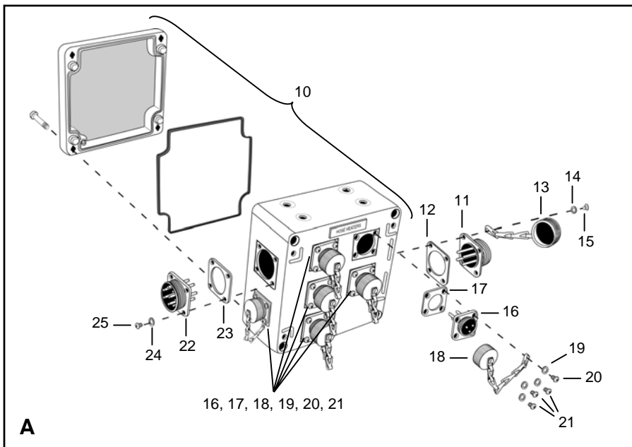
Figure 18. Electric Motor-Driven Pump Assembly P-7.
