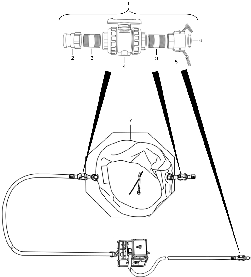
Figure 89. Cleaning Waste Storage System Adaptors.
