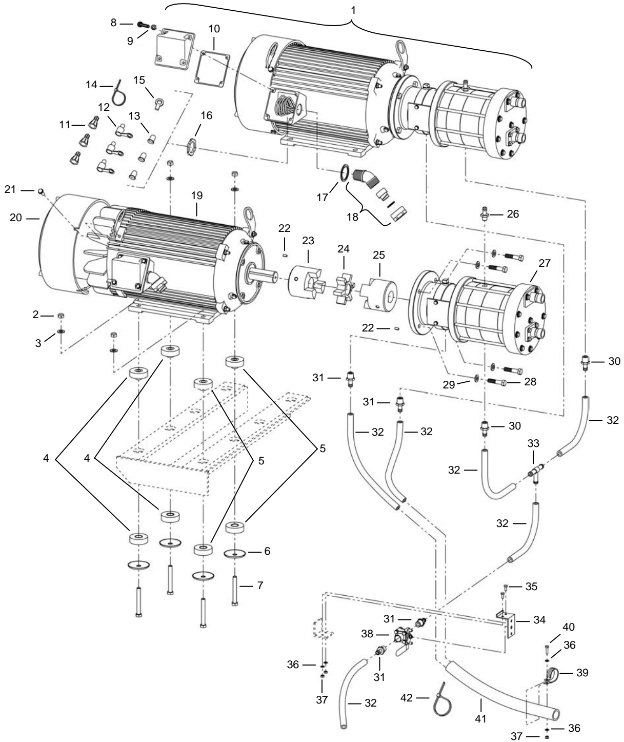
Figure 45. High Pressure Pumps P-5 and P-6 Installation.
