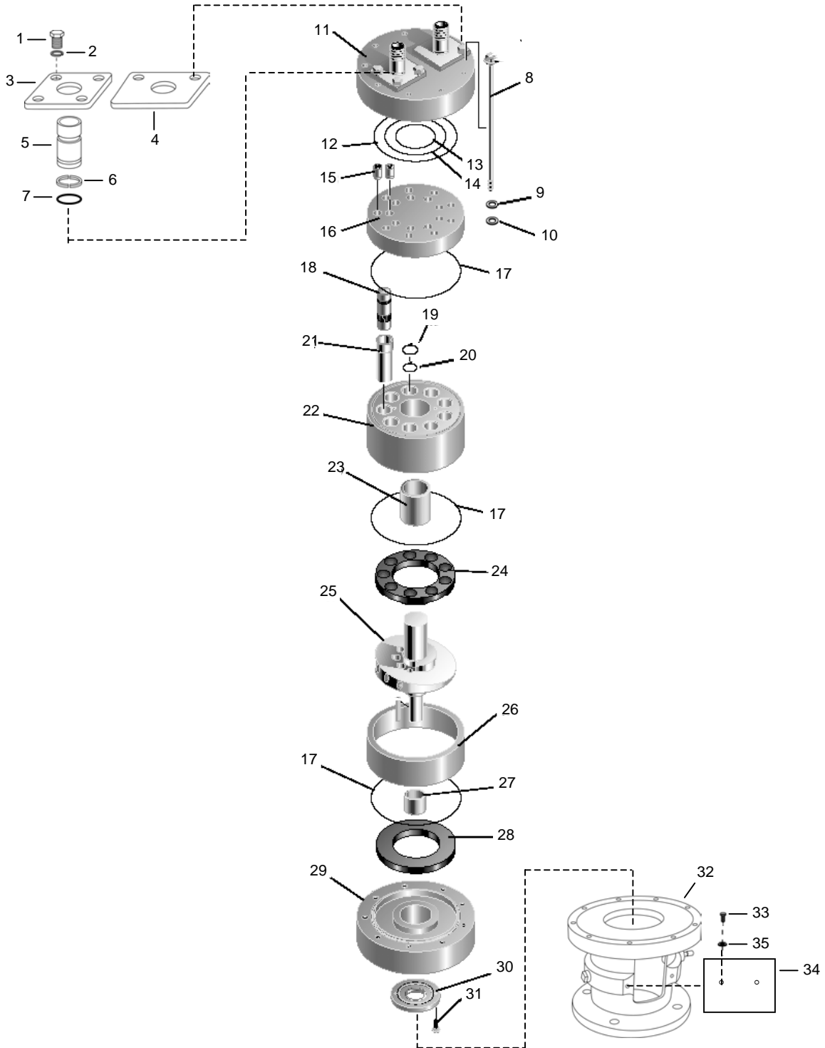
Figure 46. High Pressure Pump.
