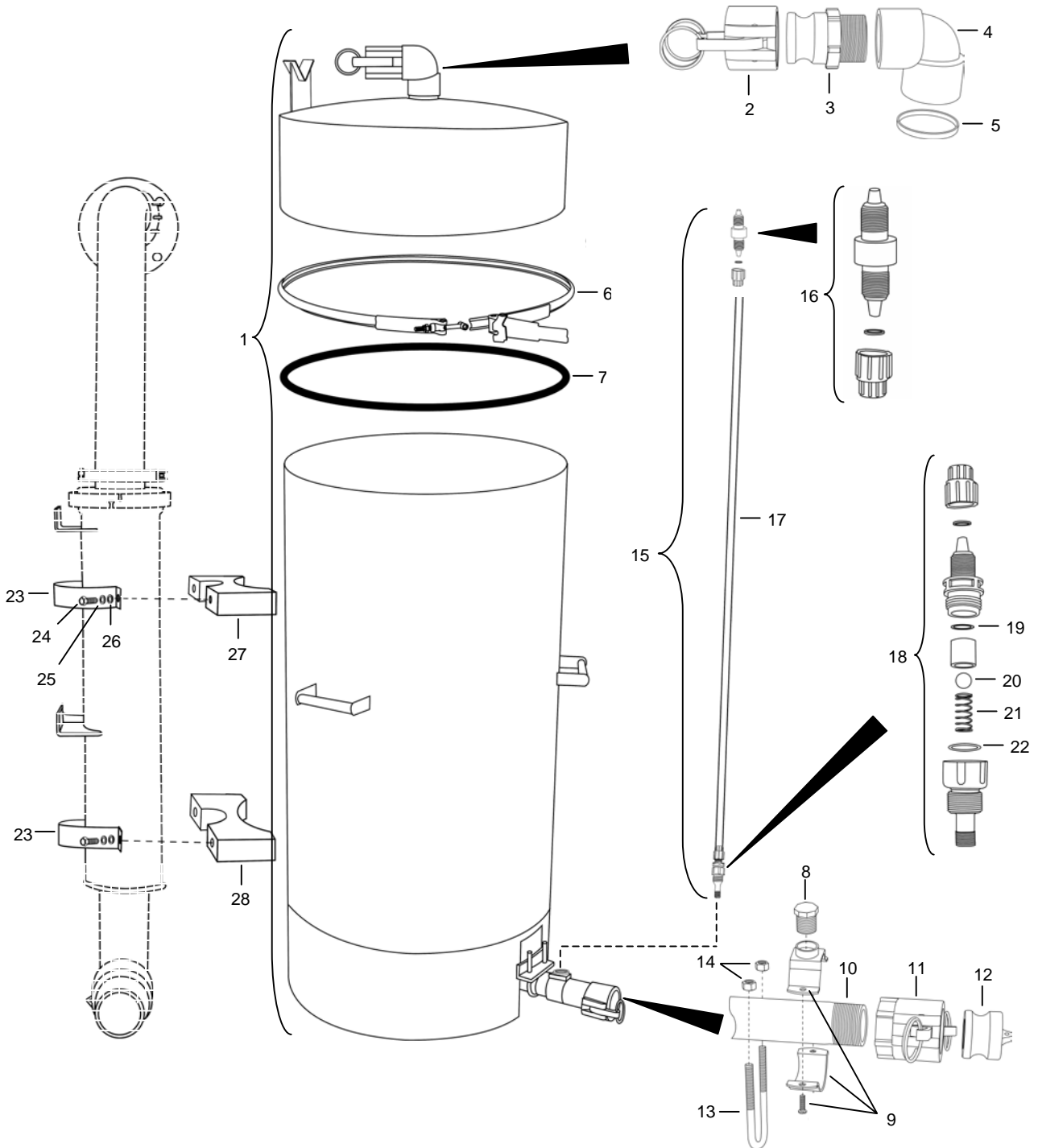
Figure 85. NBC Tank.
