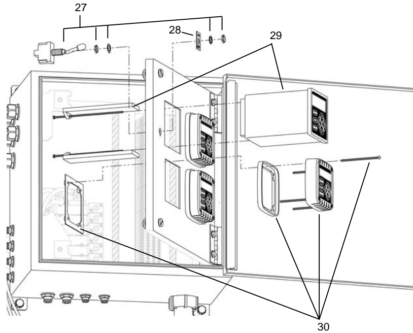
Figure 81. Instrument / Solenoid Panel (Sheet 3 of 3).
