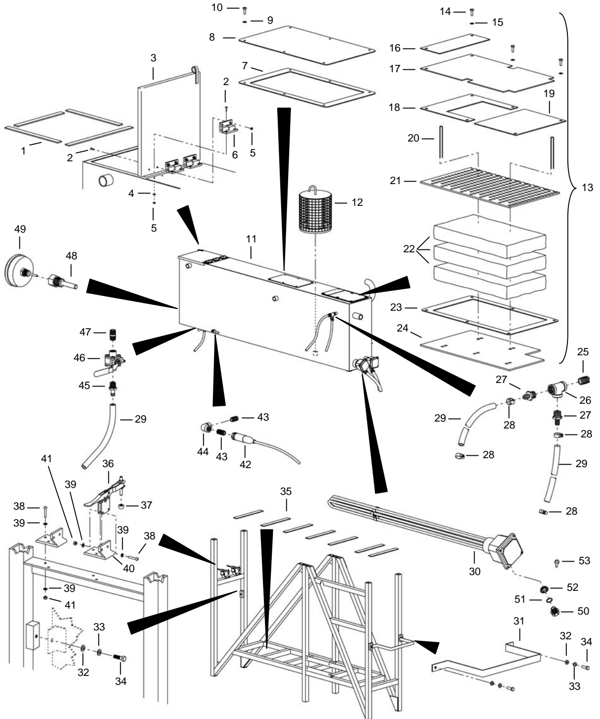
Figure 40. RO Feed Tank Assembly T-2.
