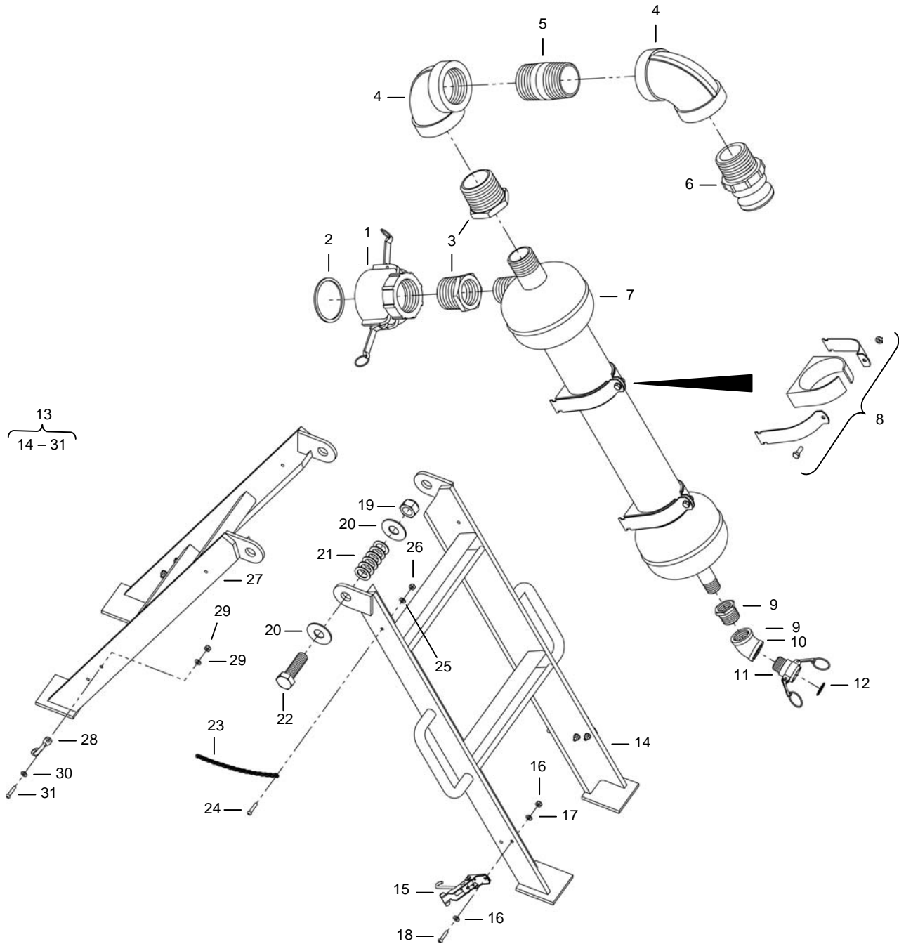
Figure 15. Cyclone Separator.
