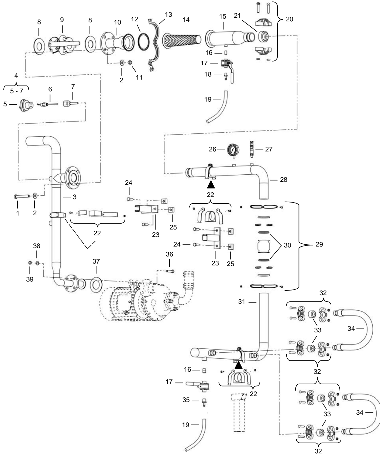
Figure 44. RO Piping Assembly M03.
